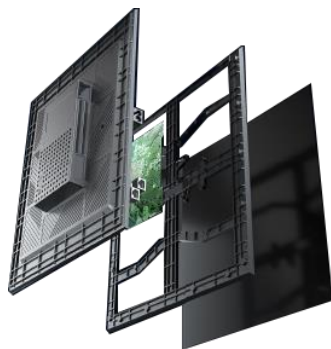
3-in-1 Module Module, PCB, Receiving Card, Power Supply, IC. In One PCB
